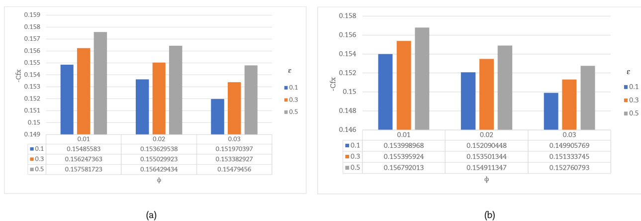
Fig. 11. Variation of (-Cf_x) for \epsilon with \phi for (a) water and (b) for Eg.
