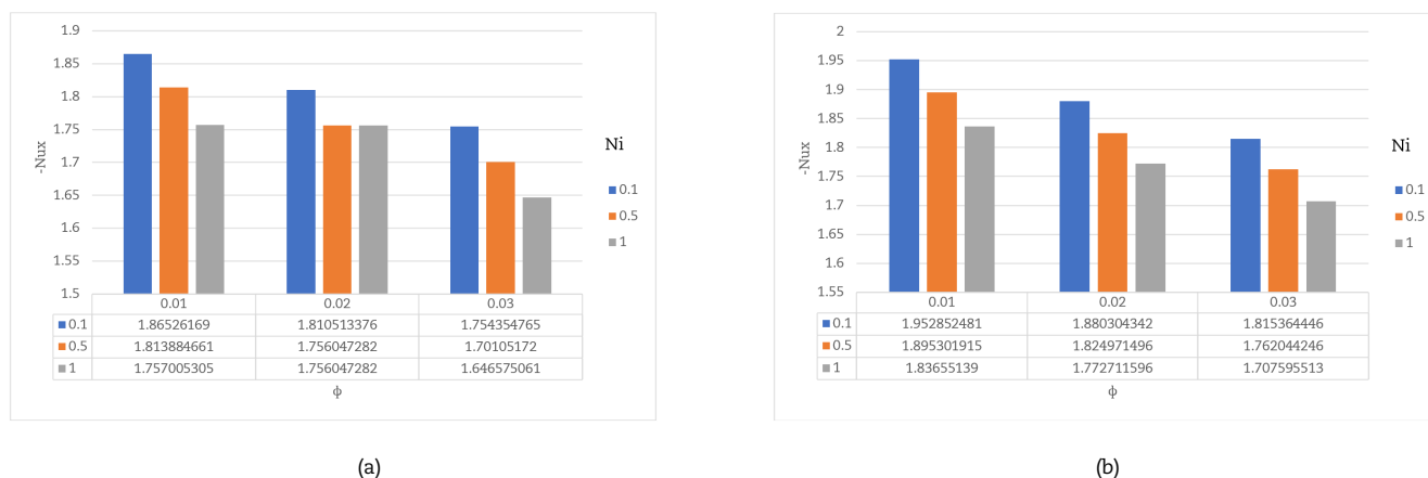
Fig. 12. Influence of Ni on Nu_x in (a) water and (b) in Eg.
